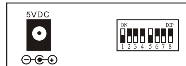
Figure 2. Media Converter Series Rear Panel
