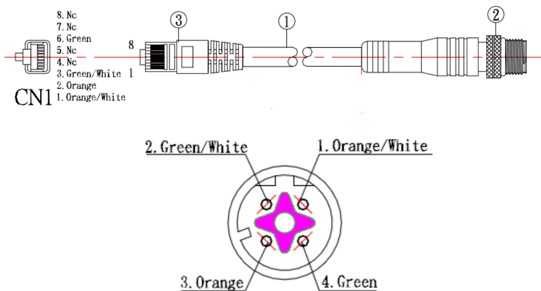
Pin assignment of M12 10/100Tx network connector
