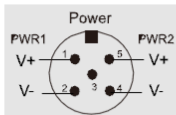
Pin assignment of Power input
