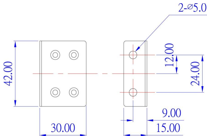
Figure-5: Wall-Mount Bracket Dimensions
