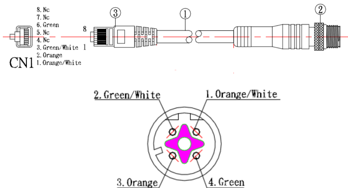
Pin assignment of M12 10/100Tx network connector
