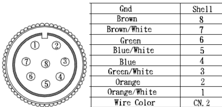
Pin assignment of M12 10/100/100T network connector
