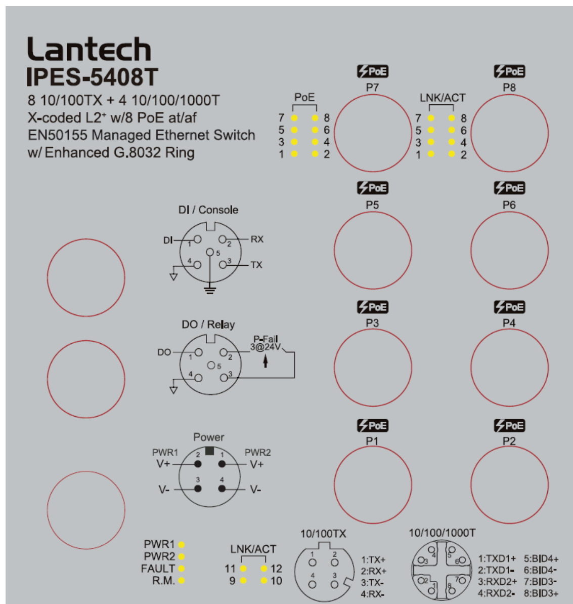
Front panel of IPES-5408T
