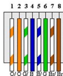
Pin assignment of M12 10/100/1000T network connector
