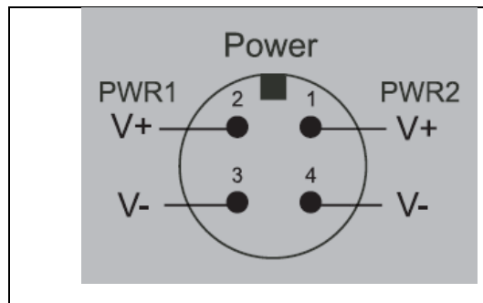
Pin assignment of Power input
